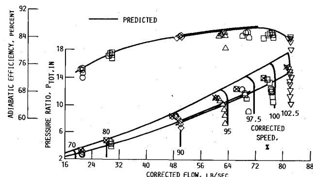
Fig. 11 Pratt & Whitney high-pressure compressor performance.
