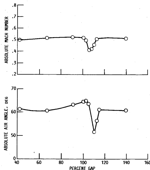
Fig. 12 Laser doppler velocimeter measurements behind ninth-stage stator (approximately midspan).
