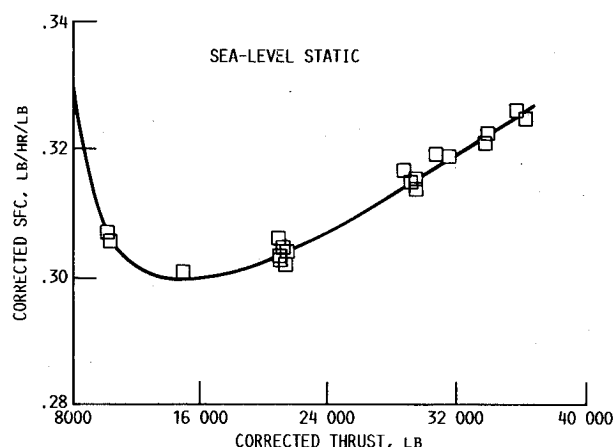
Fig. 8 Measured General Electric energy efficient engine specific fuel consumption.
