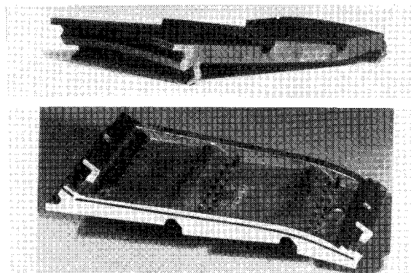
a) Counter Parallel Finwall®: turbine alloy materials, improved film and convective cooling, machined internal passages and edges.
