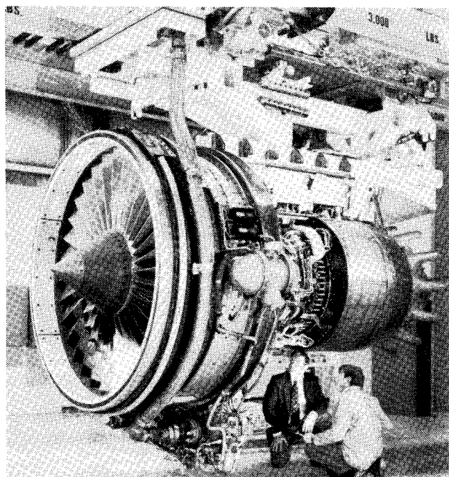
Fig. 6 General Electric energy efficient engine.
