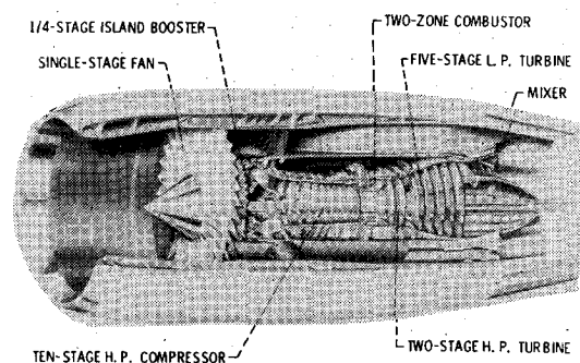
Fig. 1 General Electric energy efficient engine.
