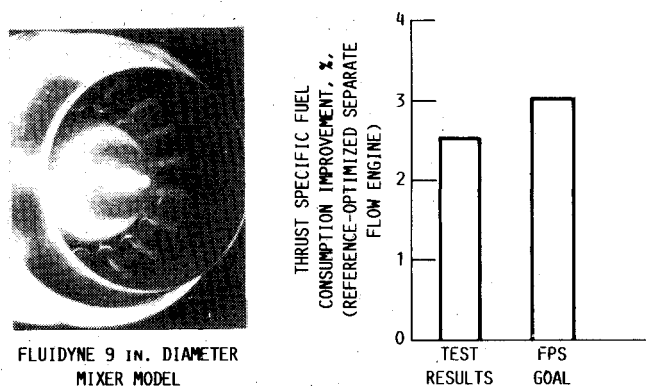
Fig. 15 Results of experimental mixer model research program.
