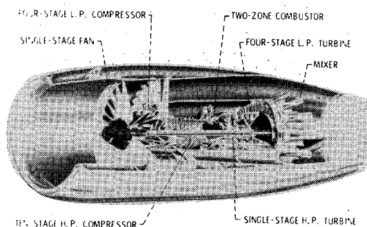
Fig. 2 Pratt & Whitney energy efficient engine.
