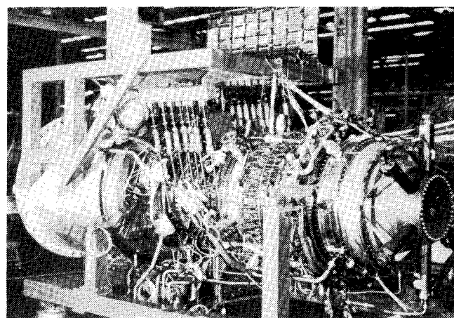
Fig. 5 Assembled General Electric core engine.
